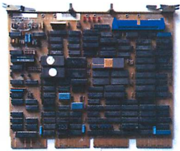
PDP-11/44 Disk Controller
